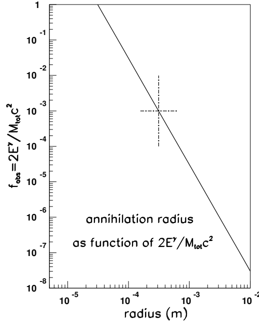
Figure 2: Photon radius R_{ann} , given by solid line as a function of the fraction of the total annihilation energy absorbed in the universe. The dot-dashed crossed lines indicate a radius of 3.16 \cdot 10^{-4} m at 2E^\gamma/M_{tot}c^2 = 10^{-3} .
