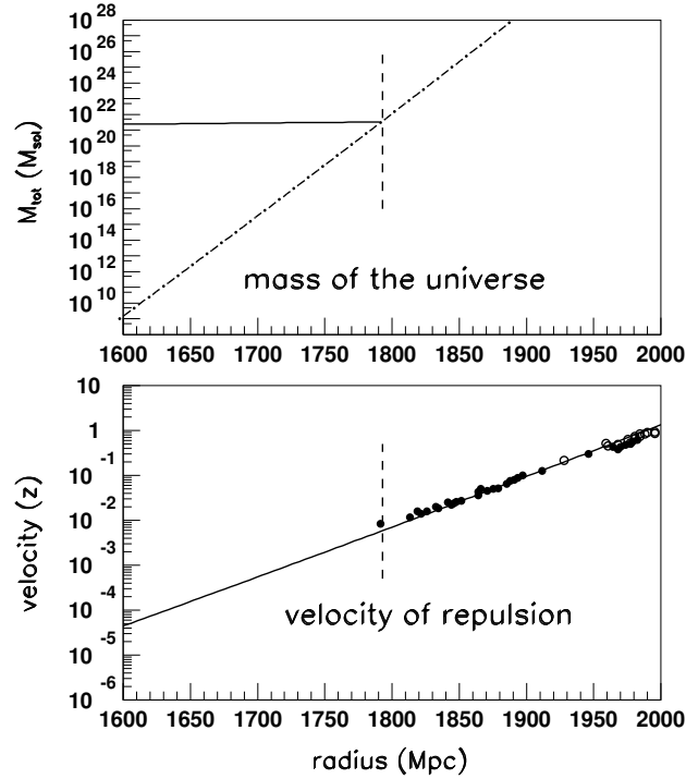
Figure 1: Upper part : Radius dependence of the calculated mass of the universe, assuming a CP-suppression factor f_{CP} = 4 \cdot 10^{-9} (dot-dashed line) in comparison with the mass deduced from the known energy density (solid line). Lower part : Radius dependence of the decay velocities in comparison with velocity-distance data from supernovae observation [1, 2]. The vertical lines indicate the effective radius R_{eff} at which the calculated gravitational mass matches that deduced from the energy density.
