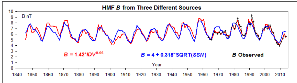
Figure 23. The Heliospheric Magnetic Field strength, B , observed (black with plus-symbols), derived from the IDV index (red) and the sunspot number (blue, version 1). There is considerable agreement (Owens et al. [2016]) about the fidelity of the IDV-derived reconstruction pioneered by Svalgaard & Cliver [2005].
