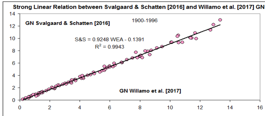
Figure 43. Because the Group Numbers are normalized to different observers (RGO and Wolfer) their values are not necessarily identical, This Figure gives the linear scaling function y = 0.925x - 0.139 ( R^2 = 0.994 ) to bring the RGO-based values onto the Wolfer scale.
