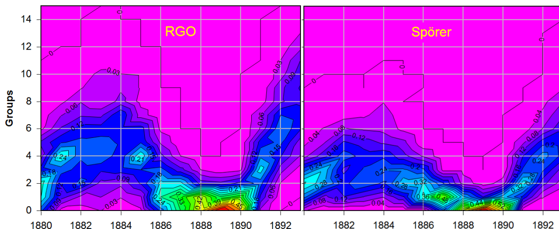
Figure 56. Frequency of occurrence of counts of groups on the solar disk as a function of time during 1880-1893 for RGO (left) and Spörer (right) determined for each year by the number of days where a given number of groups was observed on the disk divided by the number of days with an observation.
