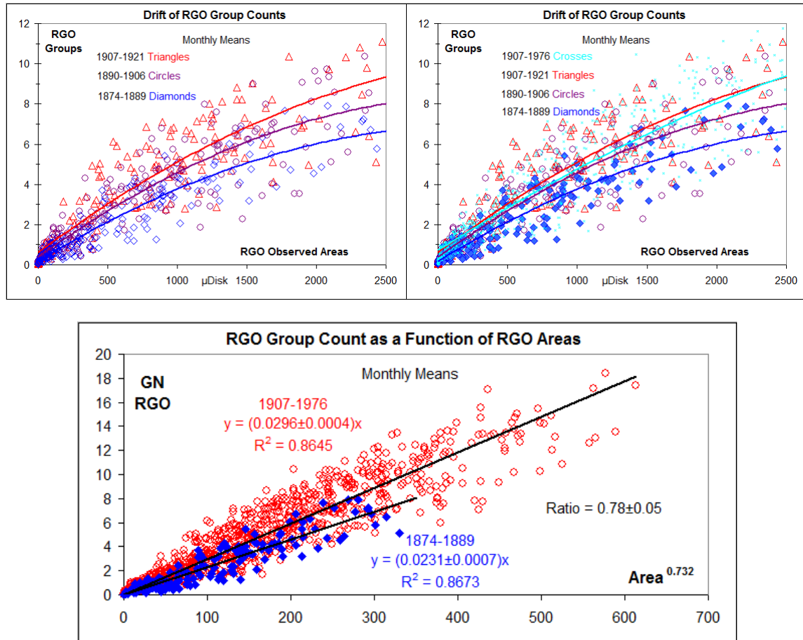
Figure 17. The number of groups reported by RGO for [left upper panel] the three intervals 1874-1889, 1890-1906, and 1907-1921. Second order polynomial fits show the progressive increases of the count for equal disk-averaged sunspot areas [observed, foreshortened; Balmaceda et al., 2009]. On the right upper panel, we have included the whole interval from 1907 until the end of the RGO data in 1976 shown as small cyan crosses. The difference in level between all that later data and the early data [blue diamonds] is manifest. The lower panel shows the RGO group count as a function of the linearized sunspot areas for the period of the drift [1874-1889, blue diamonds] and since 1907 [red dots] when the drift had abated.
